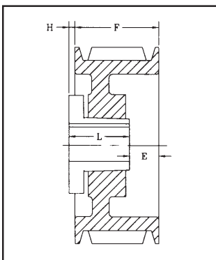
DRAWING TYPE 6 (6A, 6W)
