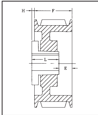
DRAWING TYPE 6 (6A, 6B, 6W)
