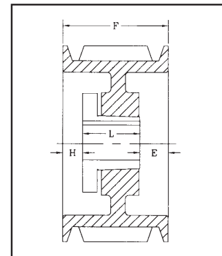
DRAWING TYPE 1 (1A, 1B, 1W)
