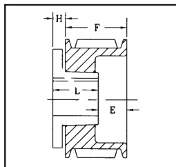
DRAWING TYPE 11 - (11B)
