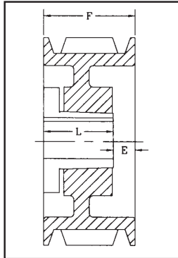
DRAWING TYPE 4 (4A, 4B, 4W)
