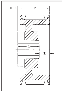
DRAWING TYPE 6 (6A, 6W)
