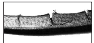
Base Cracking Cause: Loose tensioning. Belt slippage causes heat build-up and gradual under-cord hardening. Remedy: New belt. Proper tensioning.
