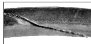
Cut Bottom & Sidewall Cause: Belt being pried over sheave during installation, as cut above indicates. Remedy: Use proper length belts and tension properly when installing.
