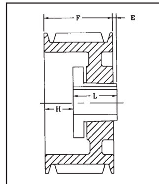
DRAWING TYPE 2 (2A, 2B, 2W)
