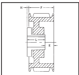
DRAWING TYPE 6 - (6A, 6B, 6W)
