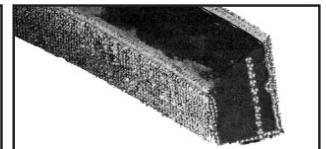
Abrasion Cause: Sidewall wear a result of foreign material and rust in sheaves. Belt dropped to bottom of sheave groove. Remedy: Dust guards to prevent abrasion.
