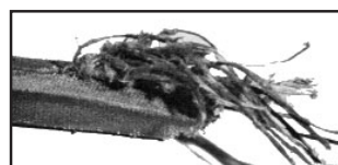
Ruptured Belt Cause: Ruptured cords in the plies, caused by high shock load on foreign object between belt and sheave groove. Remedy: Check tension, shield drive.
