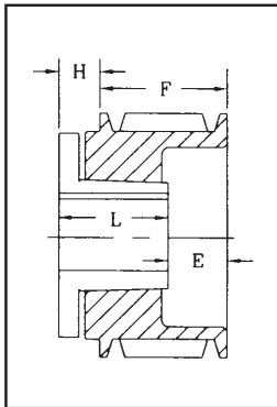
DRAWING TYPE 10 (10B)
