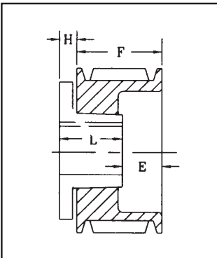
DRAWING TYPE 11 (11B)
