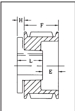
DRAWING TYPE 11 (11B)
