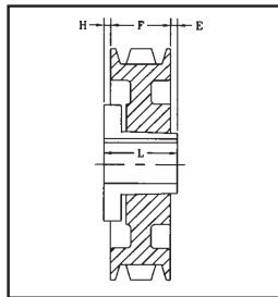
DRAWING TYPE 5 - (5A)
