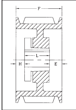
DRAWING TYPE 1 (1A, 1B, 1W)
