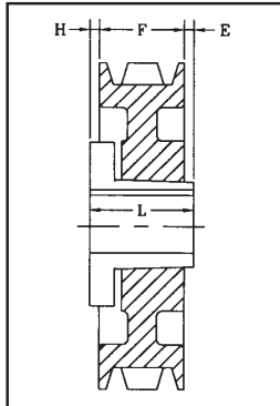
DRAWING TYPE 5 (5A, 5B)
