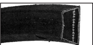
Distorted Belt Cause: Distortion caused by broken cords or adhesion breakdown. Remedy: Avoid prying on belts. Check sheaves for recommended diameters.
