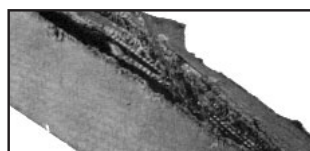
Ply Separation Cause: Split along pitch line indicating belt ran on too small diameter of sheave. Remedy: Install a (x) cogged type belt.
