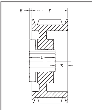
DRAWING TYPE 6 (6A)
