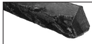
Cover Fabric Rupture Cause: Fabric covering ruptured during installation due to belt being pried over belt sheave. Remedy: Proper installation of belts.
