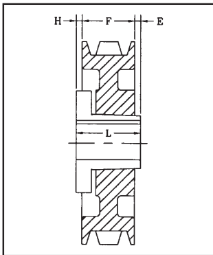
DRAWING TYPE 5 (5A, 5B, 5W)
